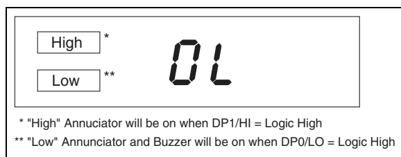
FIGURE 3-6: LCD Reading.
