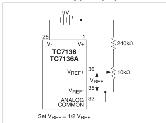
FIGURE 7-4: TC7136A INTERNAL VOLTAGE REFERENCE CONNECTION
