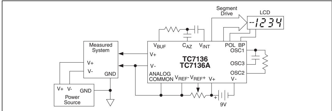
FIGURE 7-1: COMMON MODE VOLTAGE REMOVED IN BATTERY OPERATION WITH V_{IN} = \text{ANALOG COMMON}
