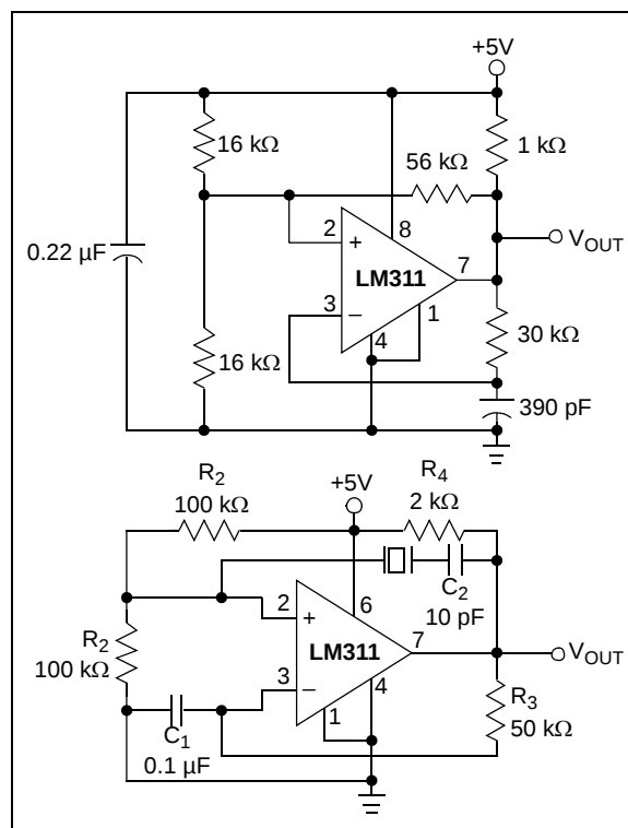
FIGURE 6-4: Comparator Clock Circuits.
