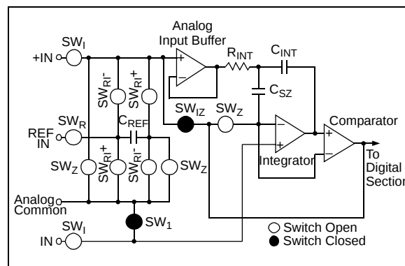
FIGURE 3-5: Integrator Output Zero Phase.
