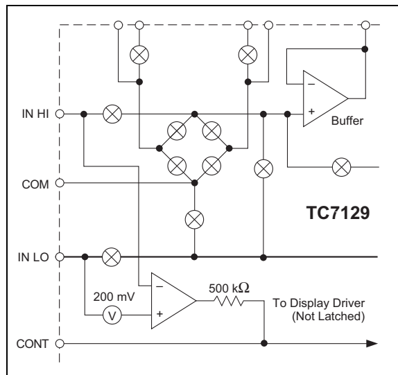
Figure 4-13: Continuity Indicator Circuit.
