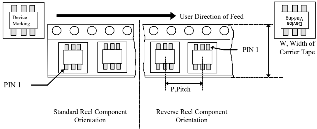
Carrier Tape, Number of Components per Reel and Reel Size
