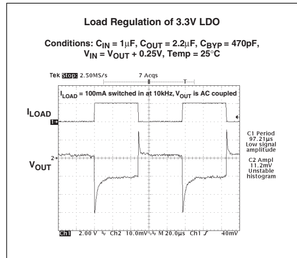
FIGURE 2-27: Load Regulation of 3.3V LDO.
