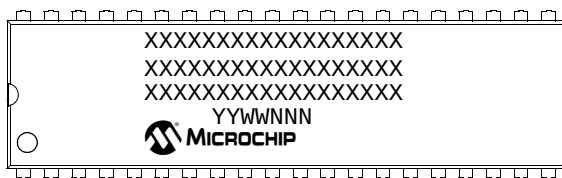
40-Pin PDIP
