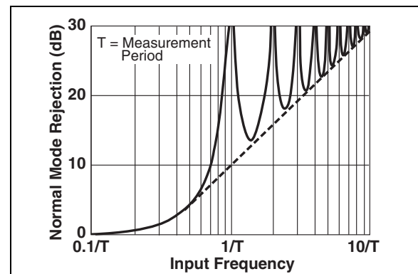
FIGURE 4-1: Integrating Converter Normal Mode Rejection.
