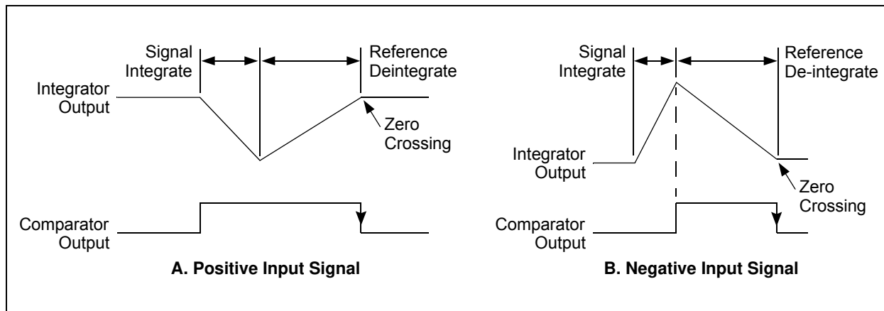
FIGURE 6-1: Comparator Output.
