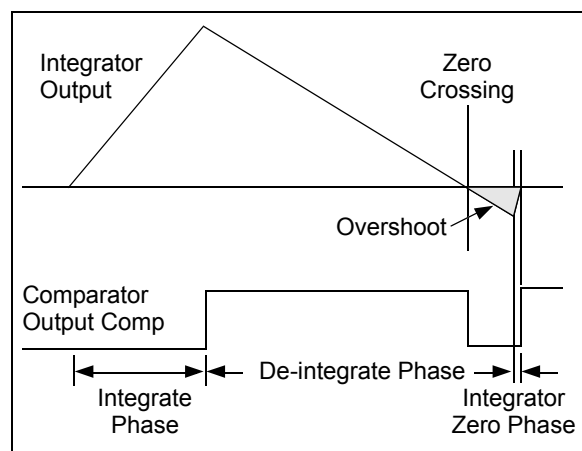
FIGURE 8-2: Overshoot.
