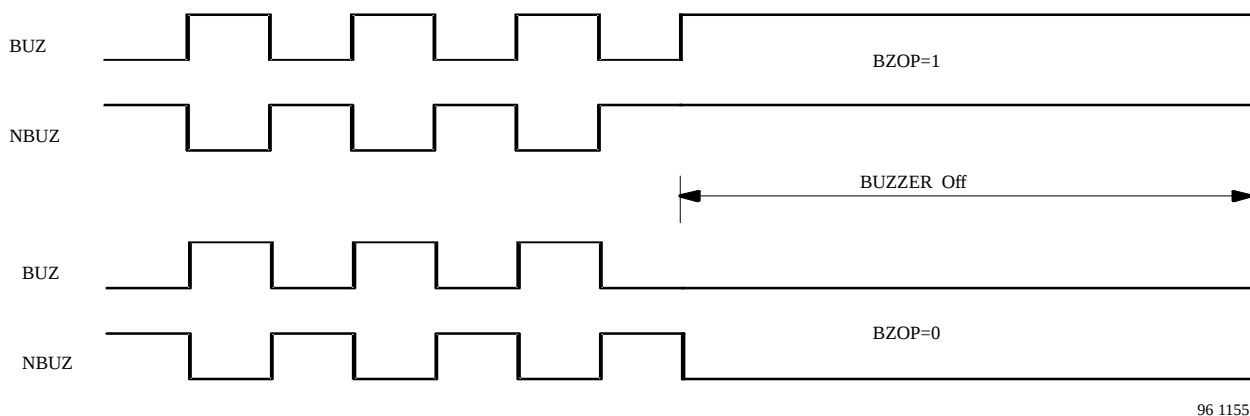
Figure 45. Buzzer waveform
