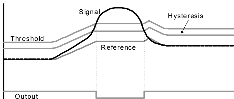
Figure 2-1 Drift Compensation
