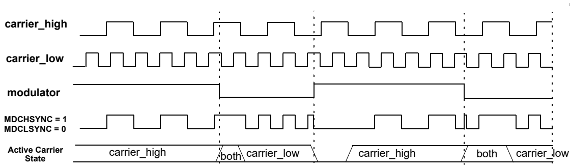
Figure 26-4. Carrier High Synchronization (MDCHSYNC = 1, MDCLSYNC = 0)
