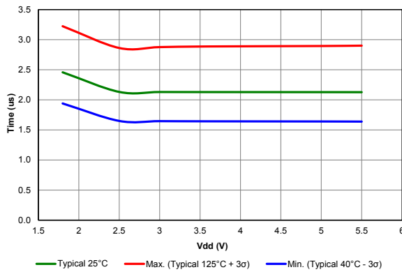
Figure 40-1. ADC RC Oscillator Period vs. Vdd
