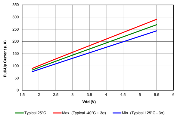
Figure 40-84. Weak Pull-Up Current
