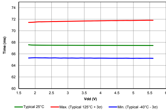
Figure 40-66. PWRT PERIOD vs. V_{DD}
