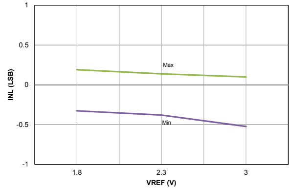
Figure 40-10. ADC 10-BIT, INL, Vdd = 3.0V, TAD = 1uS, Min and Max values at 125C + 3σ
