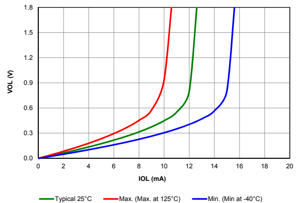
Figure 40-81. VOL vs. IOL OVER TEMPERATURE, VDD = 1.8V
