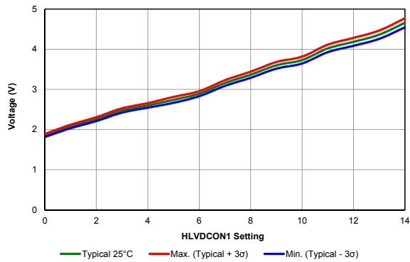
Figure 40-60. LVD Comparator Output High Trip Points
