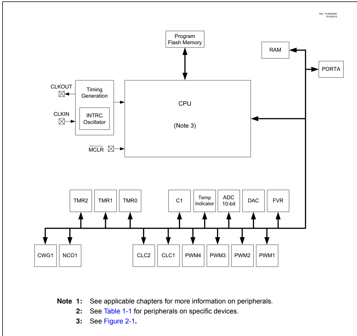
FIGURE 1-1: PIC12(L)F1501 BLOCK DIAGRAM
