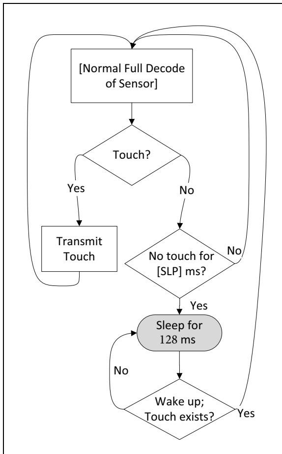
FIGURE 8-1: SLEEP FUNCTIONALITY
