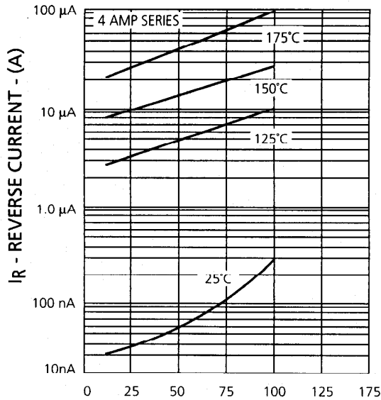
FIGURE 3 Typical Reverse Current vs. Applied Reverse Voltage
