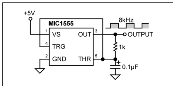
FIGURE 5-3: MIC1555 Oscillator Configuration.
