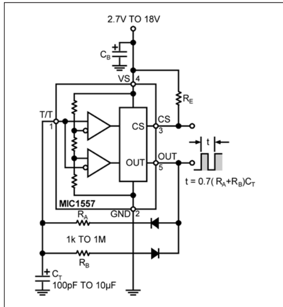
FIGURE 5-2: Oscillator Diagram.
