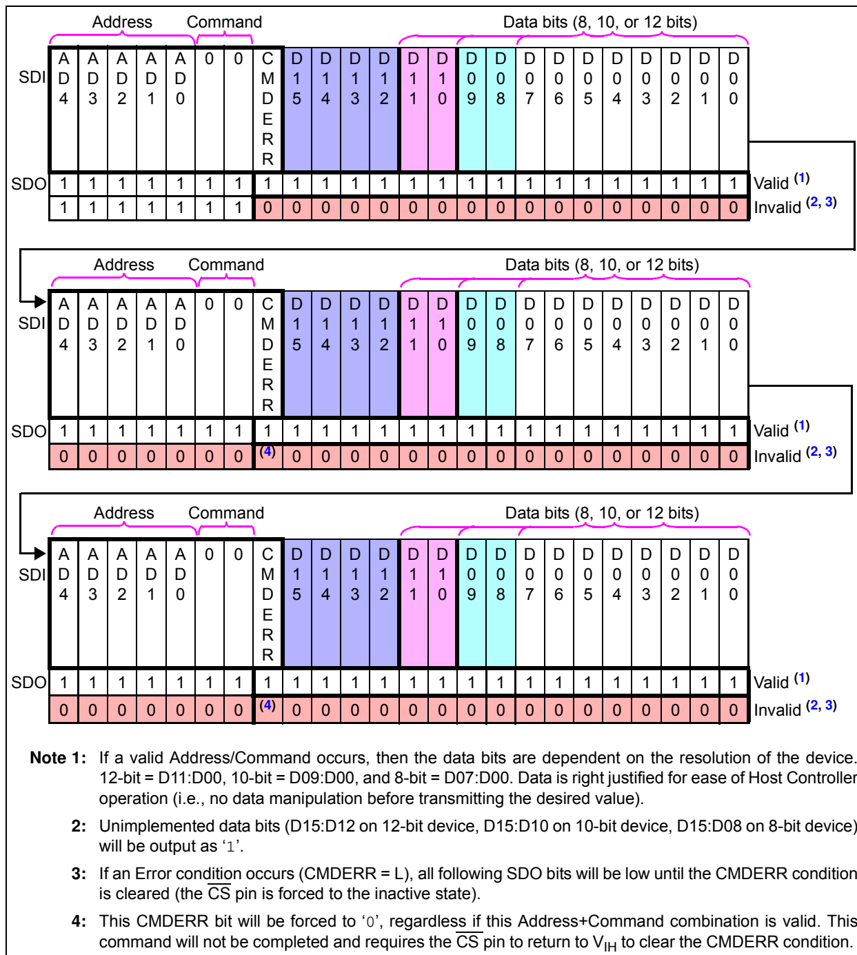
FIGURE 7-3: Continuous Write Sequence.
