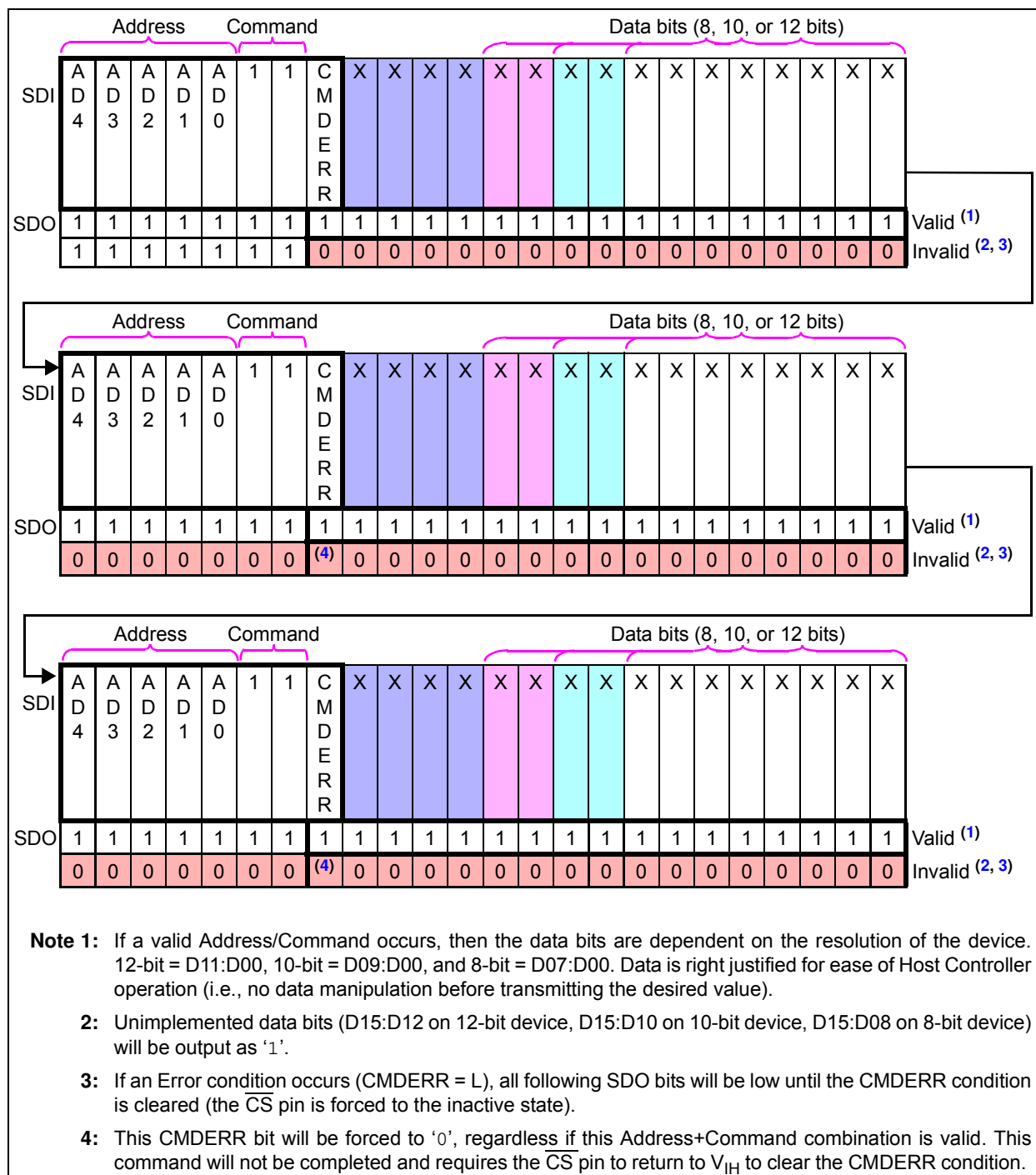
FIGURE 7-7: Continuous-Reads Sequence.
