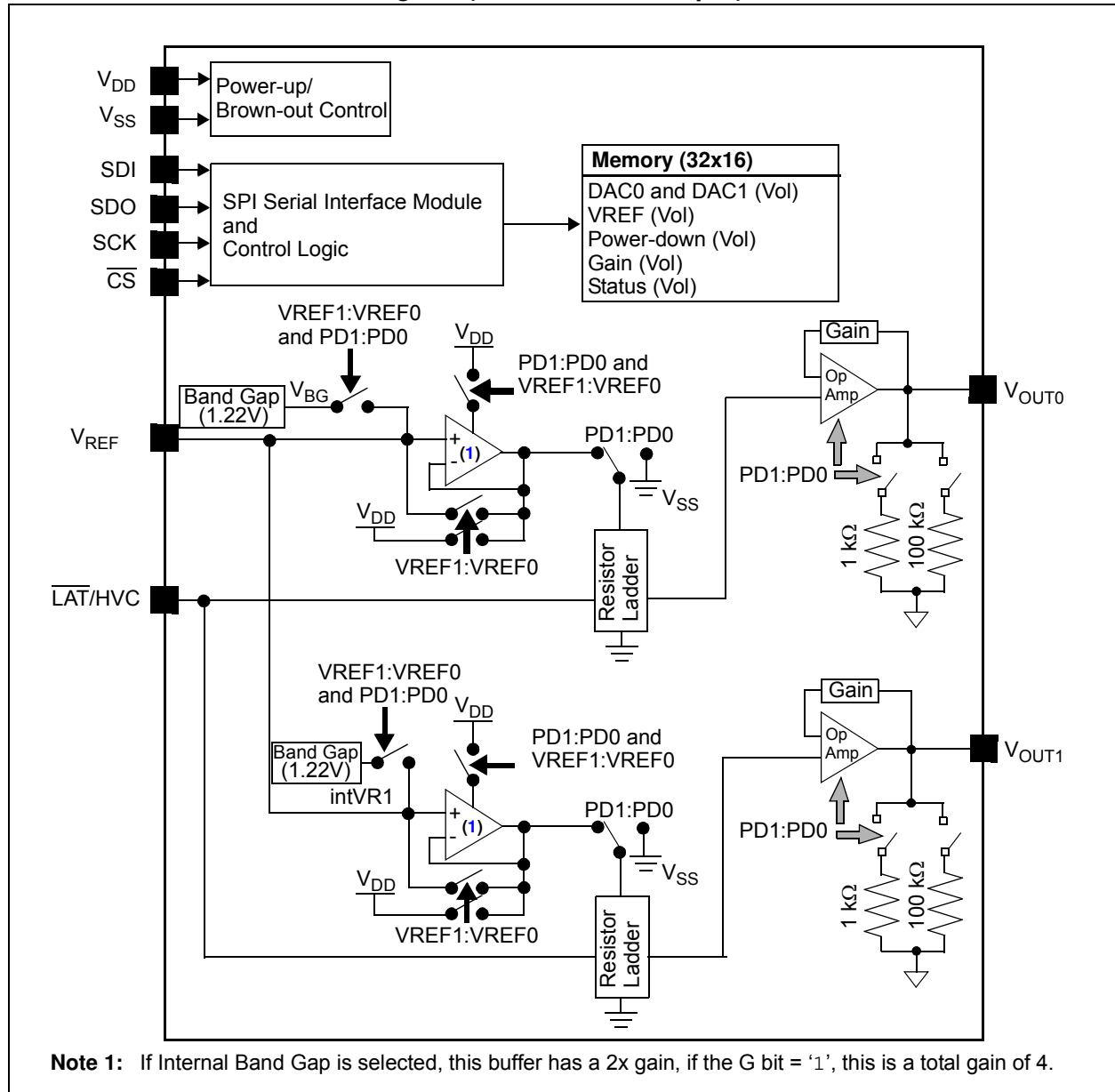
MCP48FVBX2 Device Block Diagram (Dual-Channel Output)
