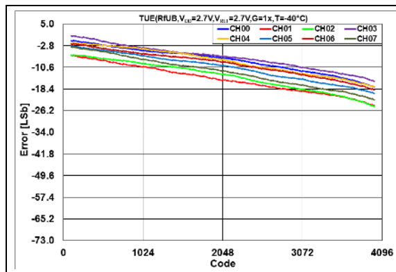
FIGURE 2-59: Total Unadjusted Error ( V_{OUT} ) vs. DAC Code, T = -40^\circ\text{C} , V_{DD} = 2.7\text{V} .
