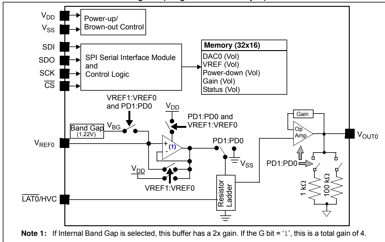
MCP48FVBX1 Device Block Diagram (Single-Channel Output)
