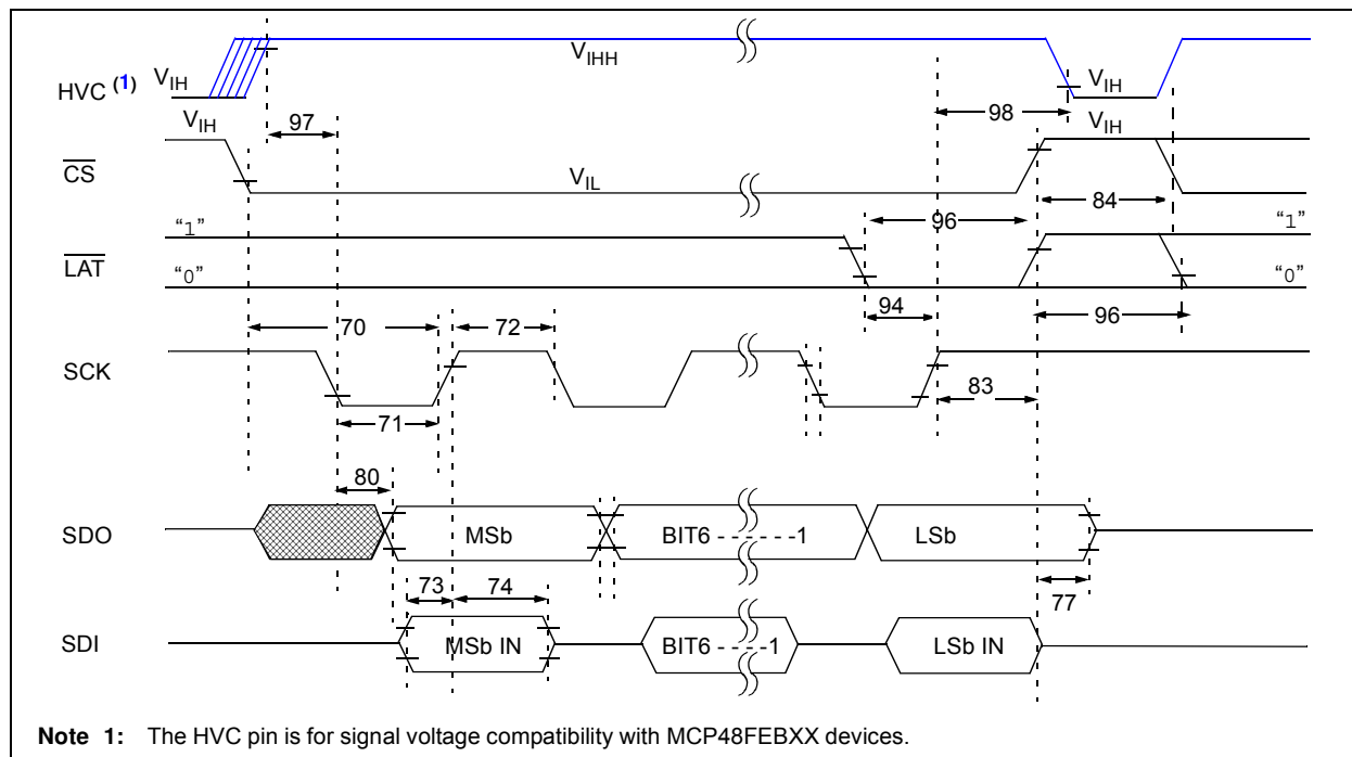
FIGURE 1-4: SPI Timing (Mode = 11) Waveforms.
