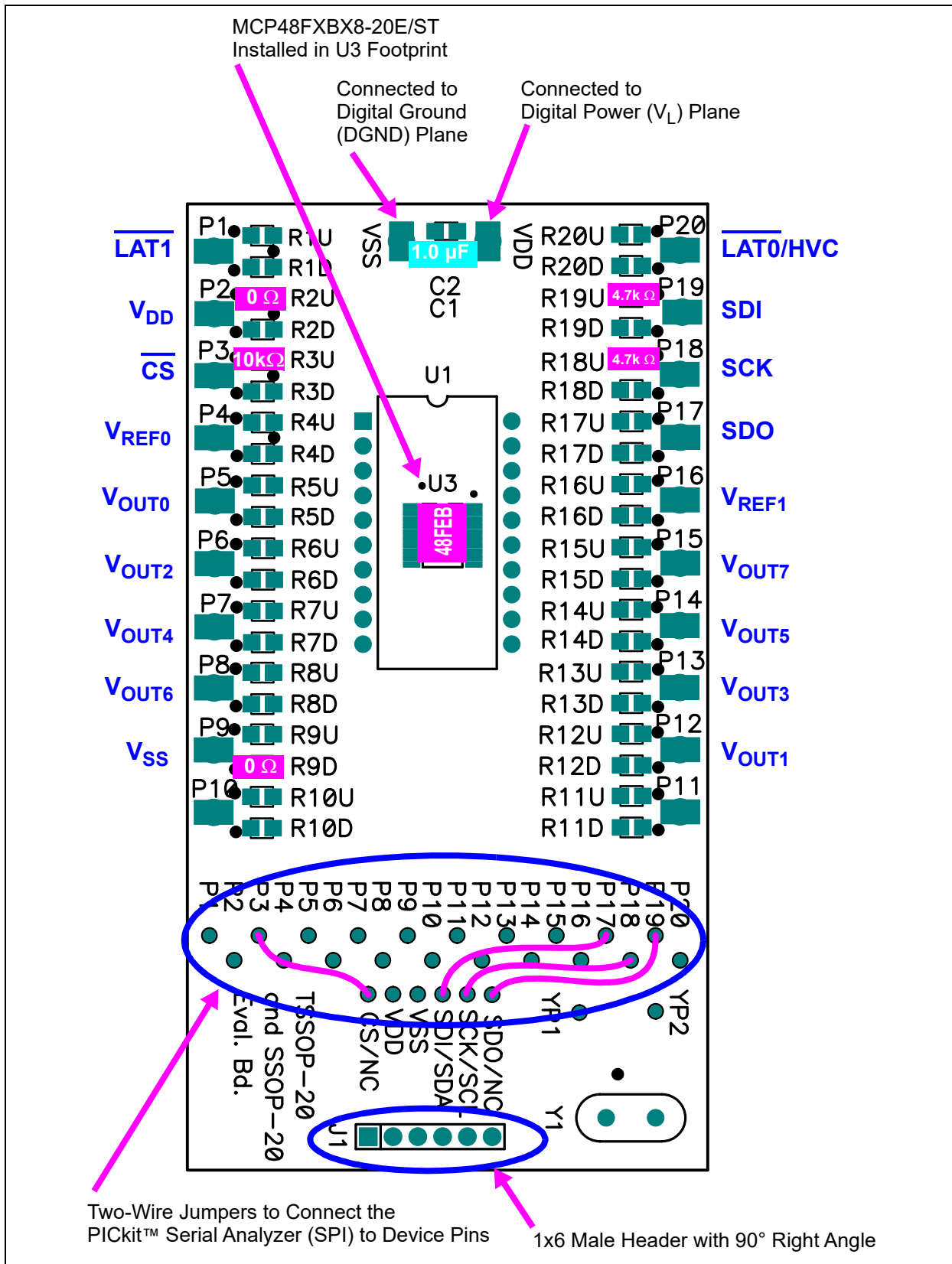
FIGURE 9-1: MCP48FVBX4/8 Evaluation Board Circuit Using TSSOP20EV.
