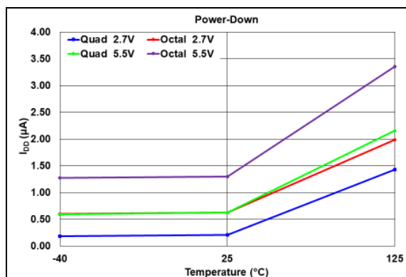
FIGURE 2-10: Power-Down Currents.
