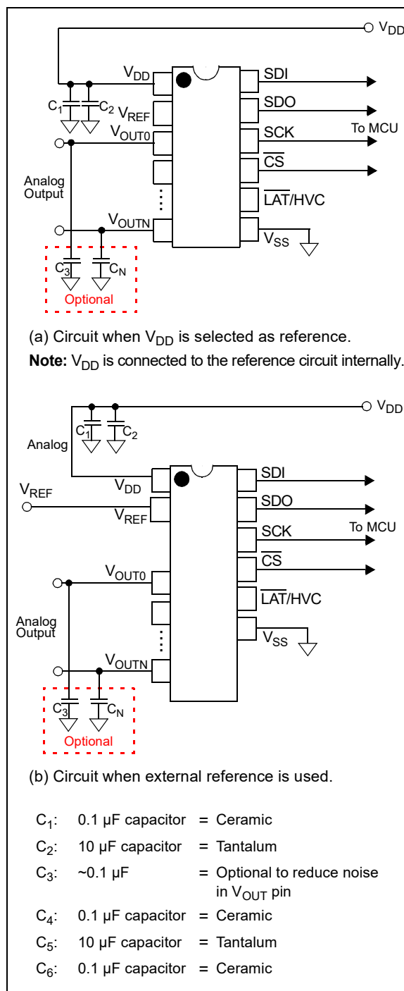
FIGURE 8-1: Example Circuit.
