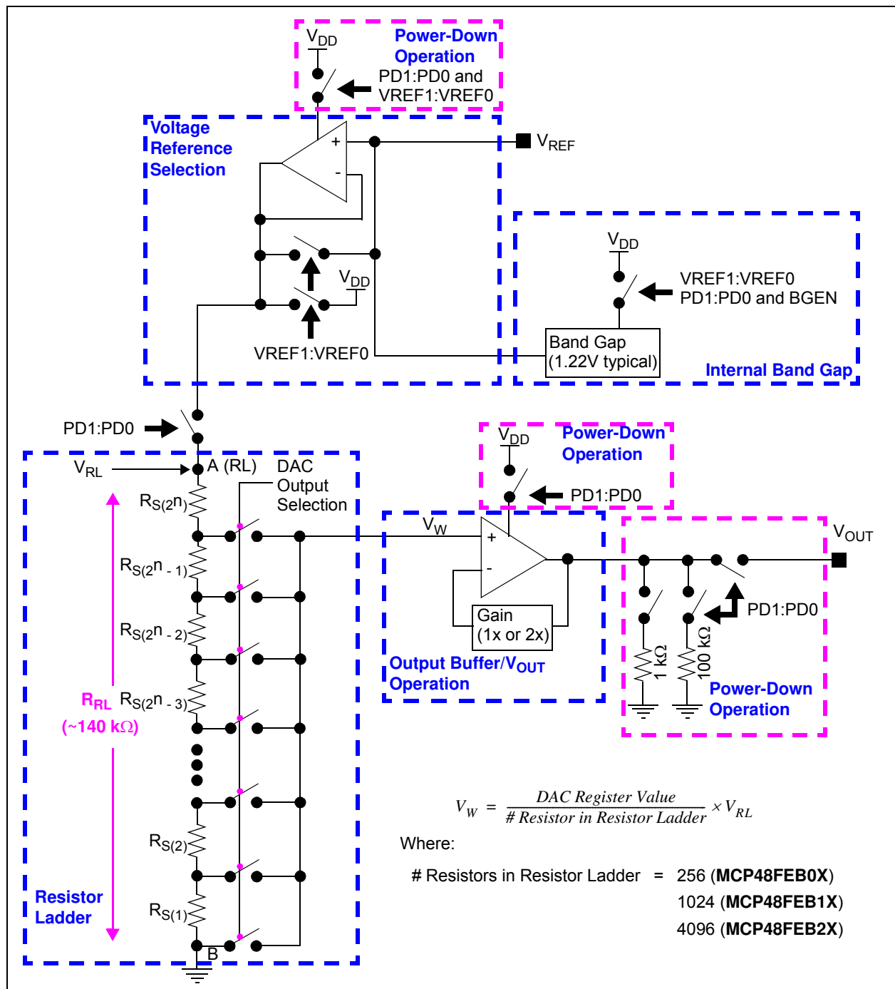
FIGURE 5-1: MCP48FEBXX DAC Module Block Diagram.
