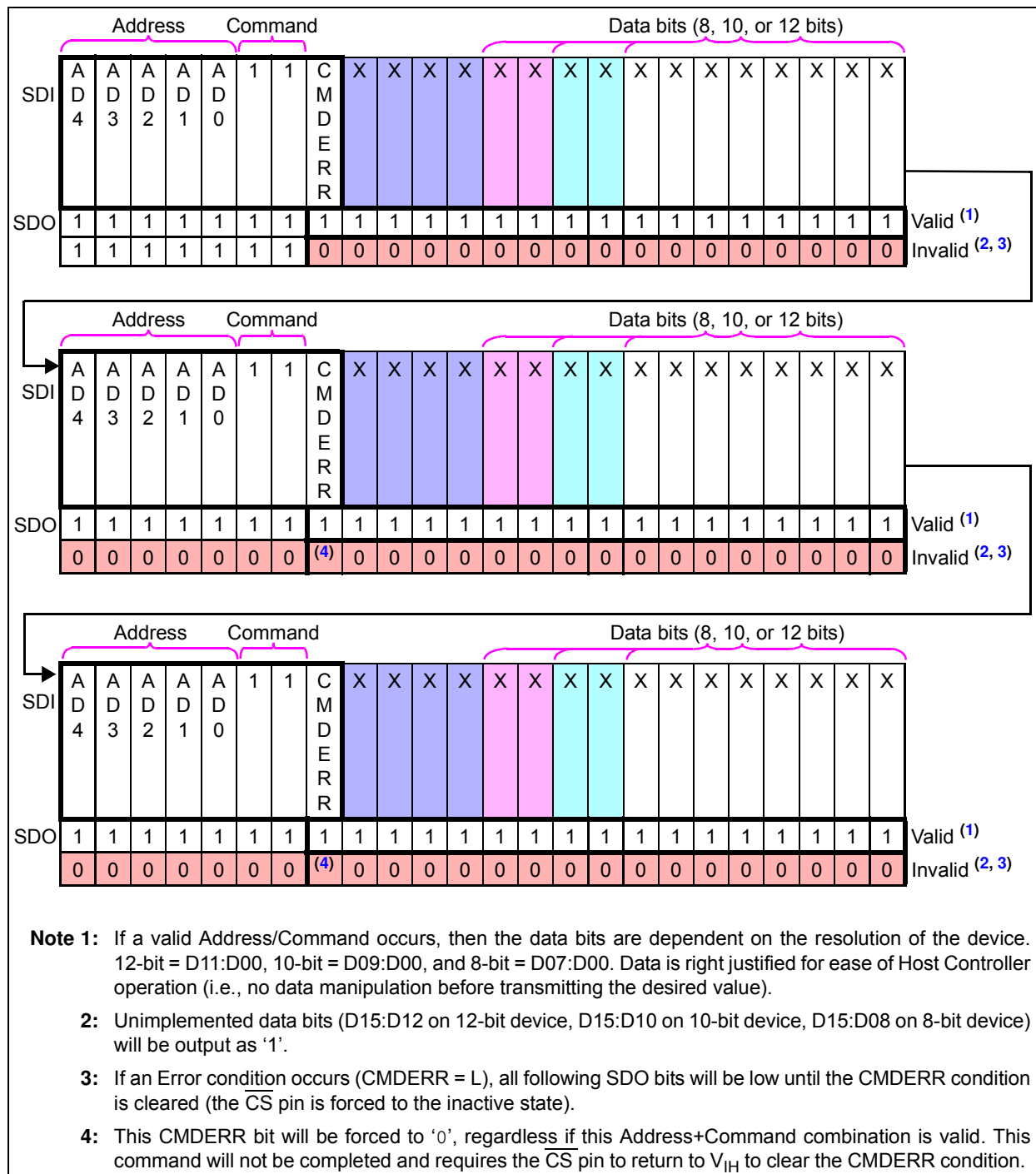
FIGURE 7-8: Continuous-Reads Sequence.
