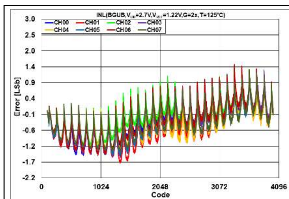
FIGURE 2-43: INL Error vs. DAC Code, T = +125^\circ\text{C} , V_{DD} = 2.7\text{V} .
