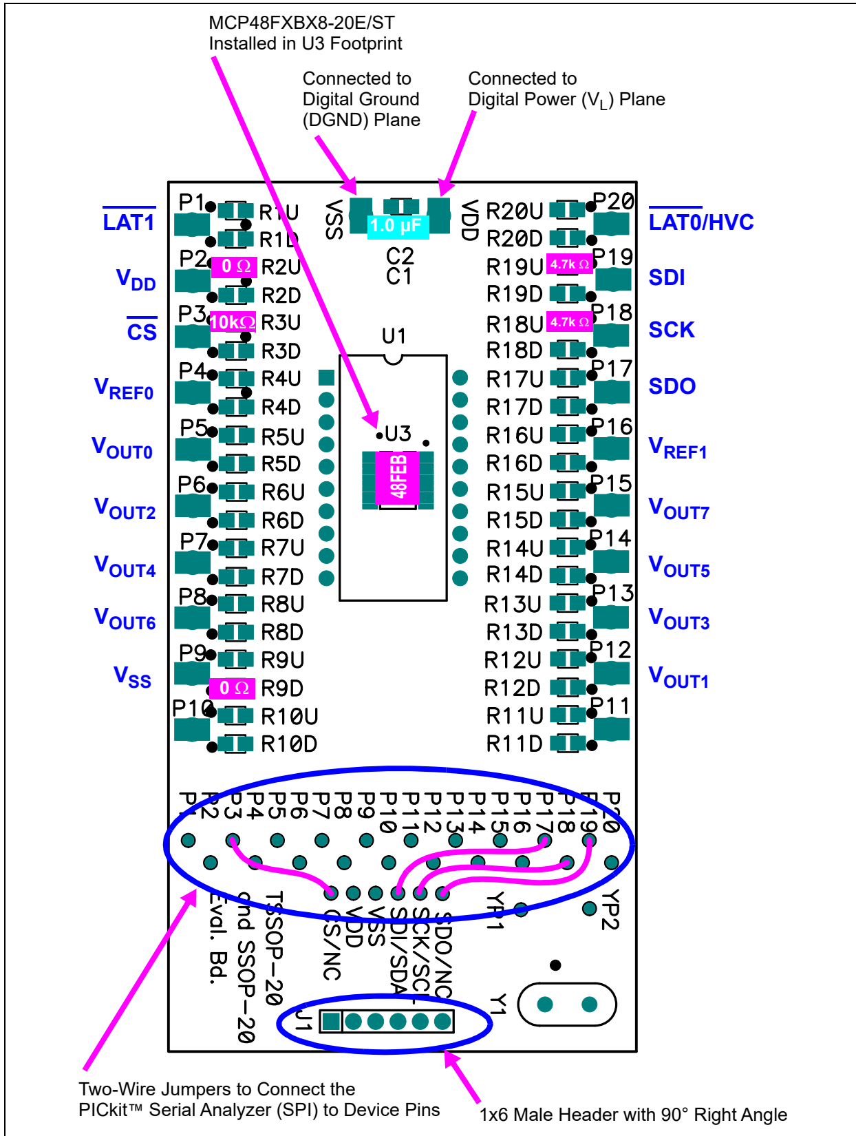
FIGURE 9-1: MCP48FXBX4/8 Evaluation Board Circuit Using TSSOP20EV.
