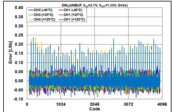
FIGURE 2-68: DNL Error vs. DAC Code and Temperature, V_{DD} = 2.7\text{V} , V_{REF} = 1.35\text{V} , G = 2\text{x} .
