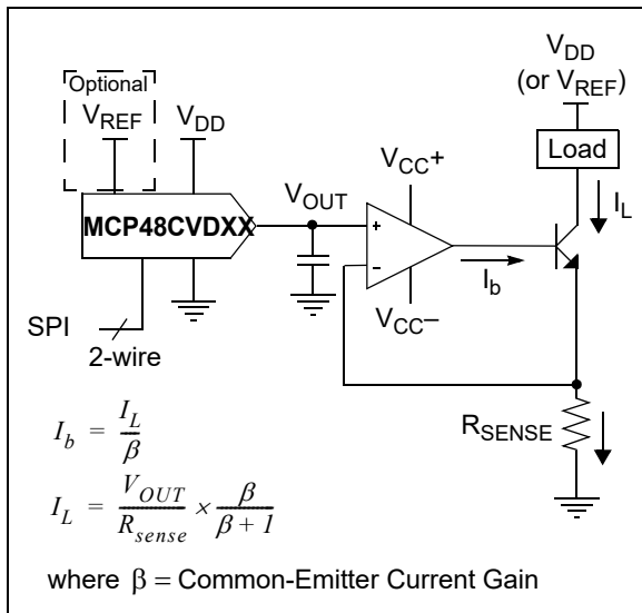
FIGURE 8-7: Digitally-Controlled Current Source.
