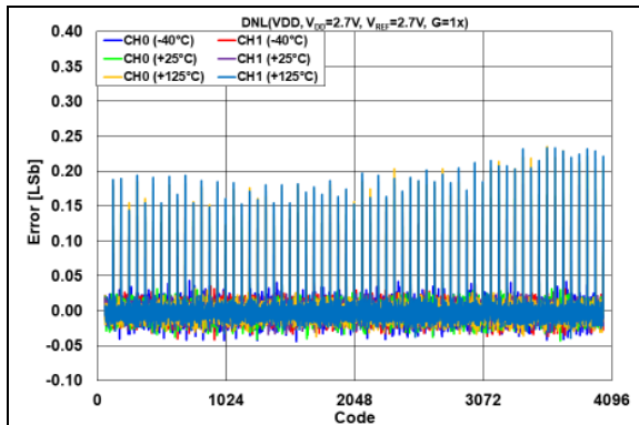
FIGURE 2-55: DNL Error vs. DAC Code and Temperature, V_{REF} = V_{DD} = 2.7\text{V} , G = 1x .
