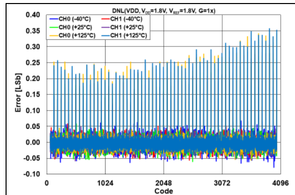
FIGURE 2-56: DNL Error vs. DAC Code and Temperature, V_{REF} = V_{DD} = 1.8\text{V} , G = 1x .
