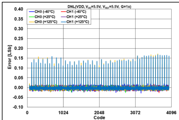
FIGURE 2-54: DNL Error vs. DAC Code and Temperature, V_{REF} = V_{DD} = 5.5\text{V} , G = 1x .
