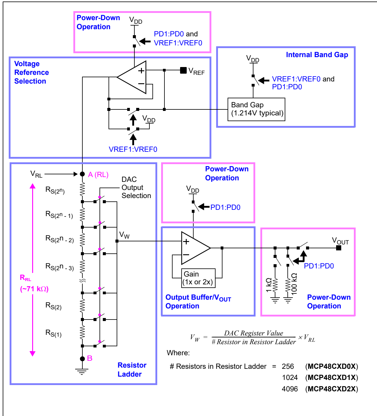
FIGURE 5-1: MCP48CXDX1/2 DAC Module Block Diagram.
