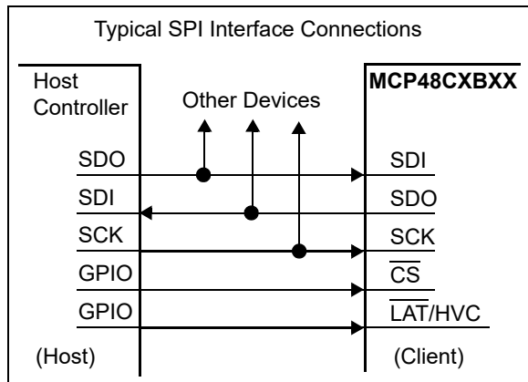
FIGURE 4-10: Typical SPI Interface.
