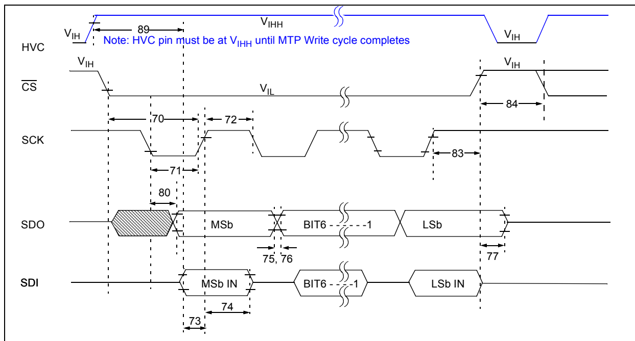
FIGURE 1-5: SPI Timing Waveform (Mode = '11').
