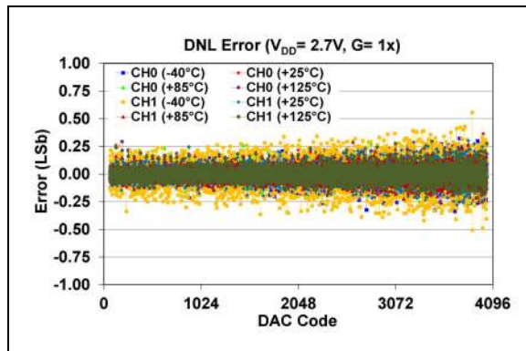
FIGURE 2-71: DNL Error vs. DAC Code and Temperature (Dual-Channel - MCP48CXB22), V_{DD} = 2.7V, Gain = 1X.
