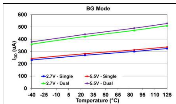
FIGURE 2-5: Average Device Supply Current - Inactive Interface ( SCK = V_{IH} or V_{IL} ) vs. Voltage and Temperature, VRxB:VRxA = '01' (Band Gap Mode).
