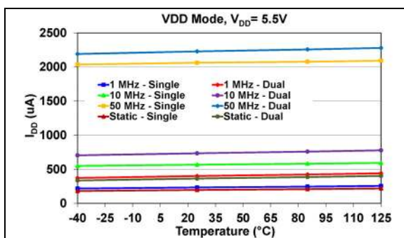
FIGURE 2-1: Average Device Supply Current vs. F_{SCK} Frequency, Voltage and Temperature - Active Interface, VRxB:VRxA = '00' , ( V_{DD} Mode).
