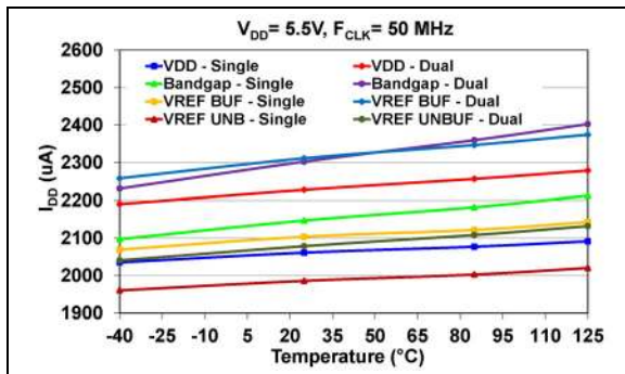
FIGURE 2-8: Average Device Supply Active Current ( I_{DDA} ) (at 5.5V and F_{SCK} = 50\text{ MHz} ) vs. Temperature and DAC Reference Voltage Mode.
