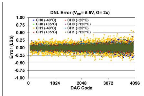
FIGURE 2-70: DNL Error vs. DAC Code and Temperature (Dual-Channel - MCP48CXB22), V_{DD} = 5.5\text{V} , Gain = 2X.
