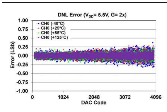
FIGURE 2-67: DNL Error vs. DAC Code and Temperature (Single-Channel - MCP48CXB21), V_{DD} = 5.5\text{V} , Gain = 2X.
