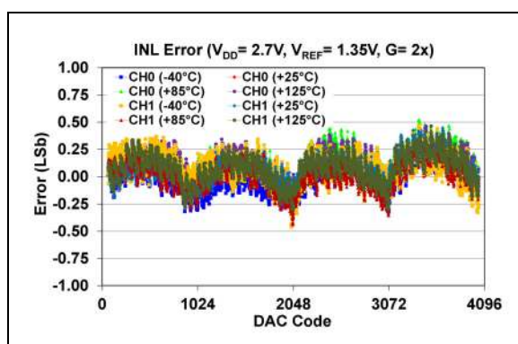
FIGURE 2-35: INL Error vs. DAC Code and Temperature (Dual-Channel - MCP48CXB22), V_{REF} = 0.5 \times V_{DD} = 1.35\text{V} , Gain = 2X.
