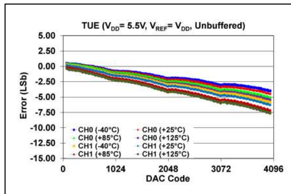
FIGURE 2-13: Total Unadjusted Error ( V_{OUT} ) vs. DAC Code and Temperature (Dual-Channel - MCP48CXB22), V_{DD} = 5.5\text{V} .
