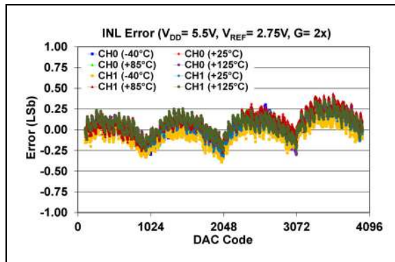
FIGURE 2-34: INL Error vs. DAC Code and Temperature (Dual-Channel - MCP48CXB22), V_{REF} = 0.5 \times V_{DD} = 2.75\text{V} , Gain = 2X.
