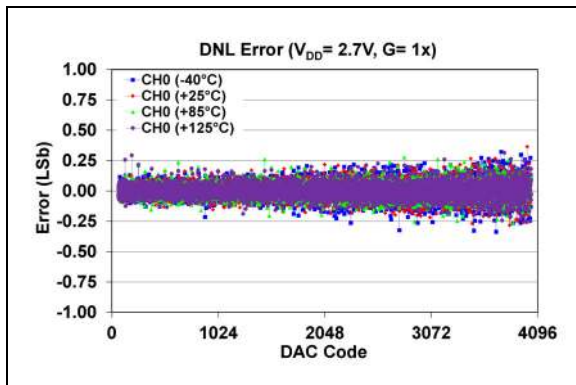
FIGURE 2-68: DNL Error vs. DAC Code and Temperature (Single-Channel - MCP48CXB21), V_{DD} = 2.7\text{V} , Gain = 1X.
