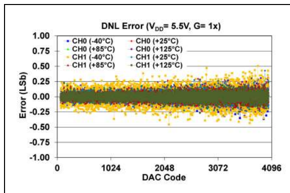
FIGURE 2-69: DNL Error vs. DAC Code and Temperature (Dual-Channel - MCP48CXB22), V_{DD} = 5.5\text{V} , Gain = 1X.
