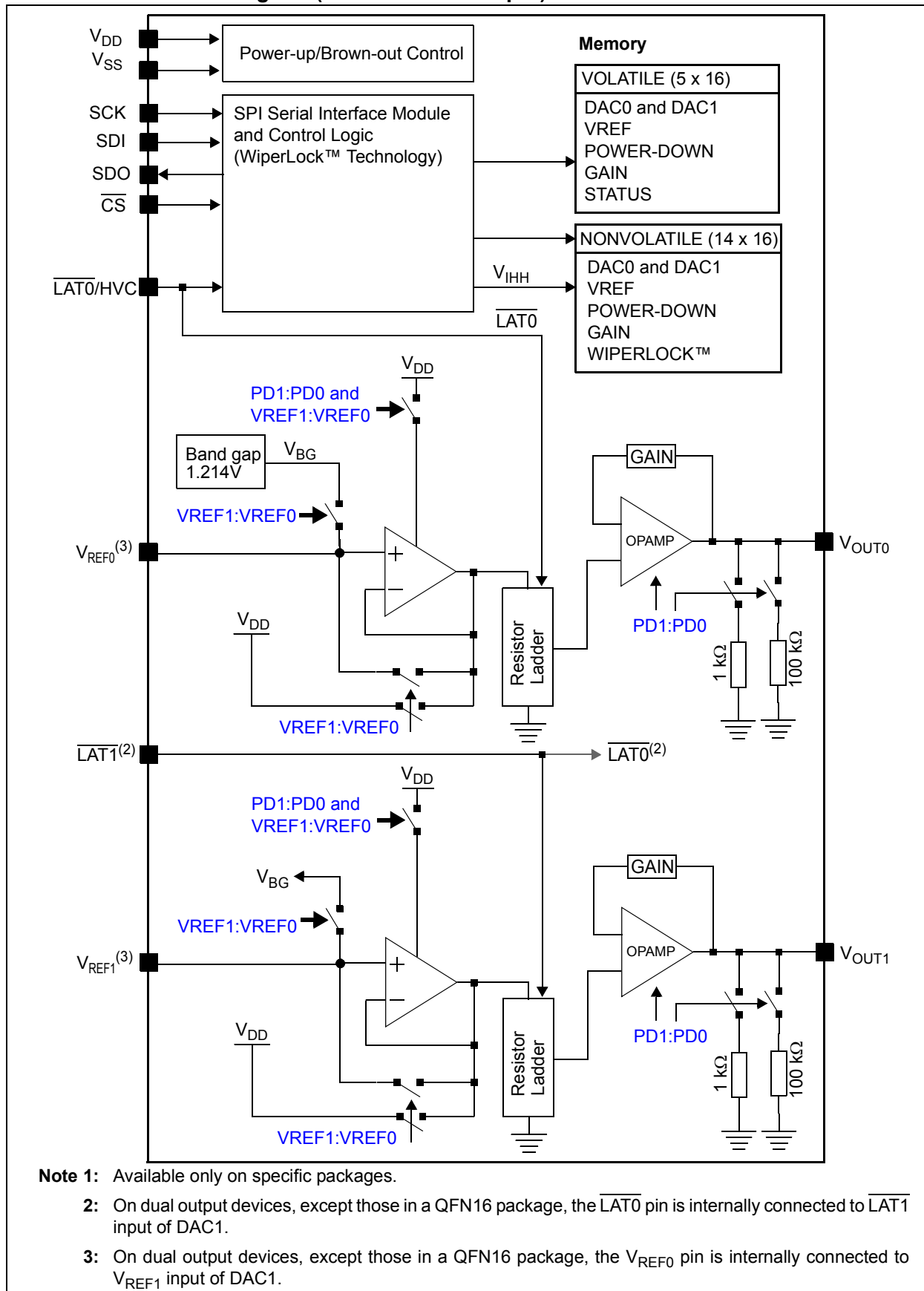
MCP48CVBX2 Block Diagram (Dual-Channel Output)
