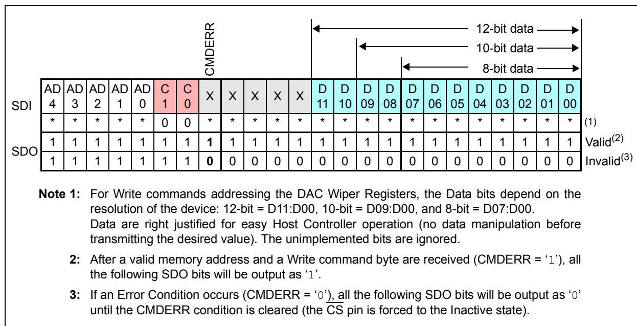
FIGURE 7-2: Write Single Memory Location Command - SDI and SDO States.
