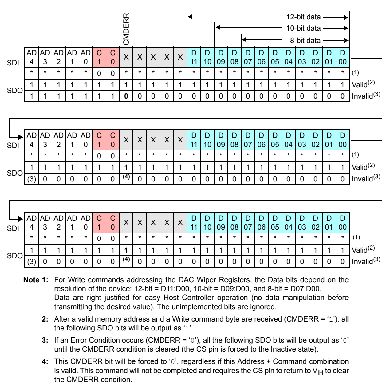
FIGURE 7-3: Continuous Write Sequence (Volatile Memory Only).
