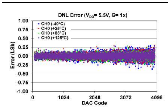
FIGURE 2-66: DNL Error vs. DAC Code and Temperature (Single-Channel - MCP48CXB21), V_{DD} = 5.5\text{V} , Gain = 1X.
