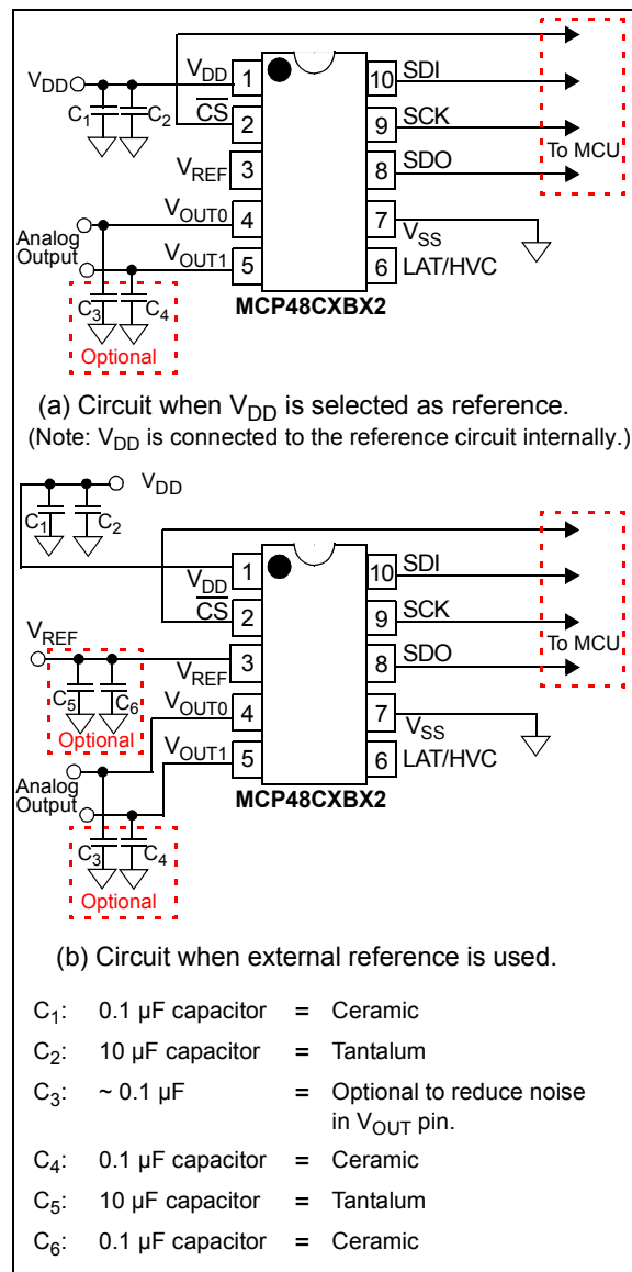
FIGURE 8-1: Example Circuit.
