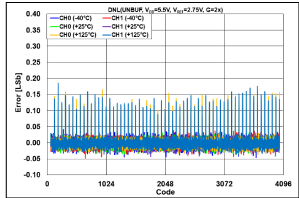
FIGURE 2-67: DNL Error vs. DAC Code and Temperature, V_{DD} = 5.5\text{V} , V_{REF} = 2.75\text{V} , G = 2\times .
