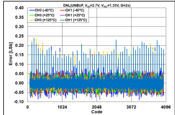
FIGURE 2-68: DNL Error vs. DAC Code and Temperature, V_{DD} = 2.7\text{V} , V_{REF} = 1.35\text{V} , G = 2\times .
