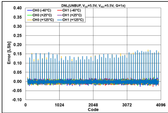
FIGURE 2-64: DNL Error vs. DAC Code and Temperature, V_{DD} = V_{REF} = 5.5\text{V} , G = 1\times .
