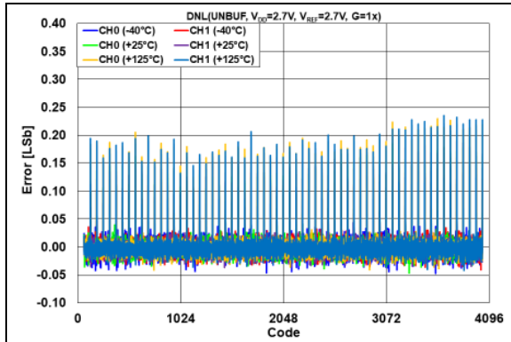
FIGURE 2-65: DNL Error vs. DAC Code and Temperature, V_{DD} = V_{REF} = 2.7\text{V} , G = 1\times .
