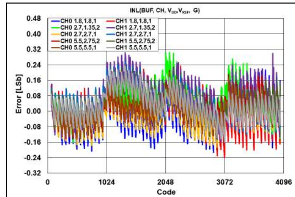
FIGURE 2-53: INL Error vs. DAC Code, Temperature = +25^\circ\text{C} .
