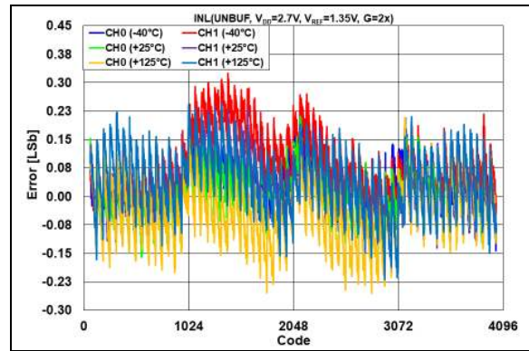
FIGURE 2-46: INL Error vs. DAC Code and Temperature, V_{DD} = 2.7\text{V} , V_{REF} = 1.35\text{V} , G = 2x .
