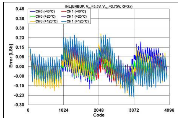
FIGURE 2-45: INL Error vs. DAC Code and Temperature, V_{DD} = 5.5\text{V} , V_{REF} = 2.75\text{V} , G = 2x .
