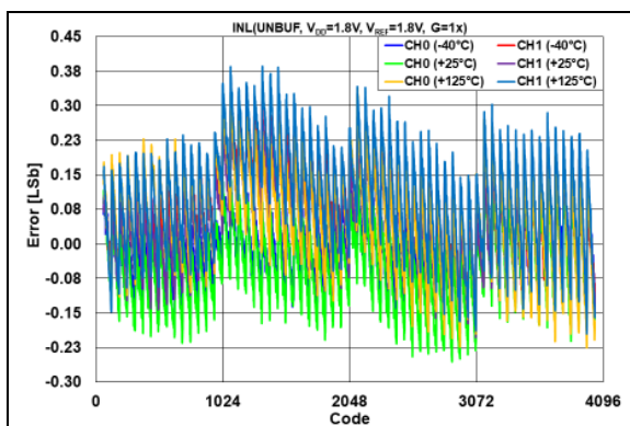
FIGURE 2-44: INL Error vs. DAC Code and Temperature, V_{DD} = V_{REF} = 1.8\text{V} , G = 1x .
