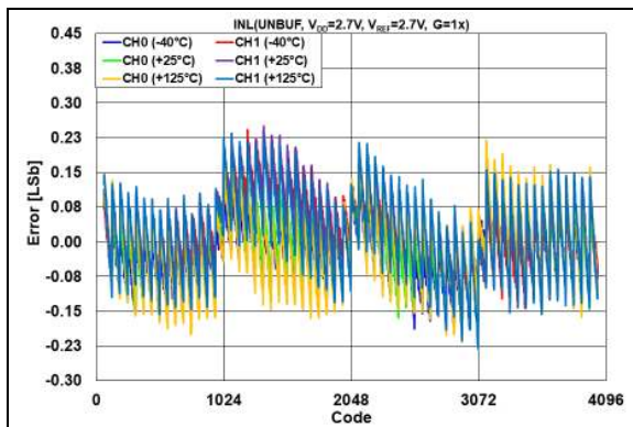
FIGURE 2-43: INL Error vs. DAC Code and Temperature, V_{DD} = V_{REF} = 2.7\text{V} , G = 1x .
