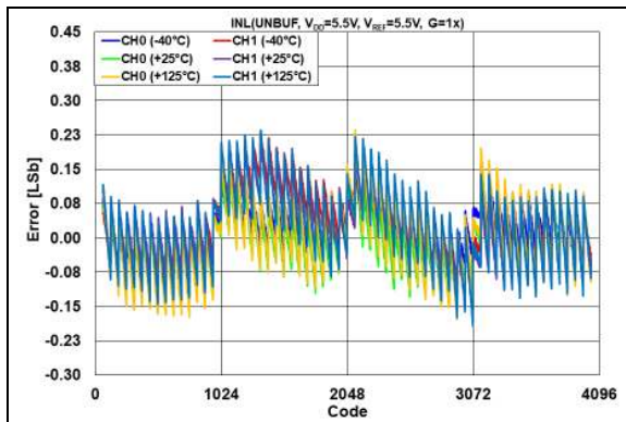
FIGURE 2-42: INL Error vs. DAC Code and Temperature, V_{DD} = V_{REF} = 5.5\text{V} , G = 1x .
