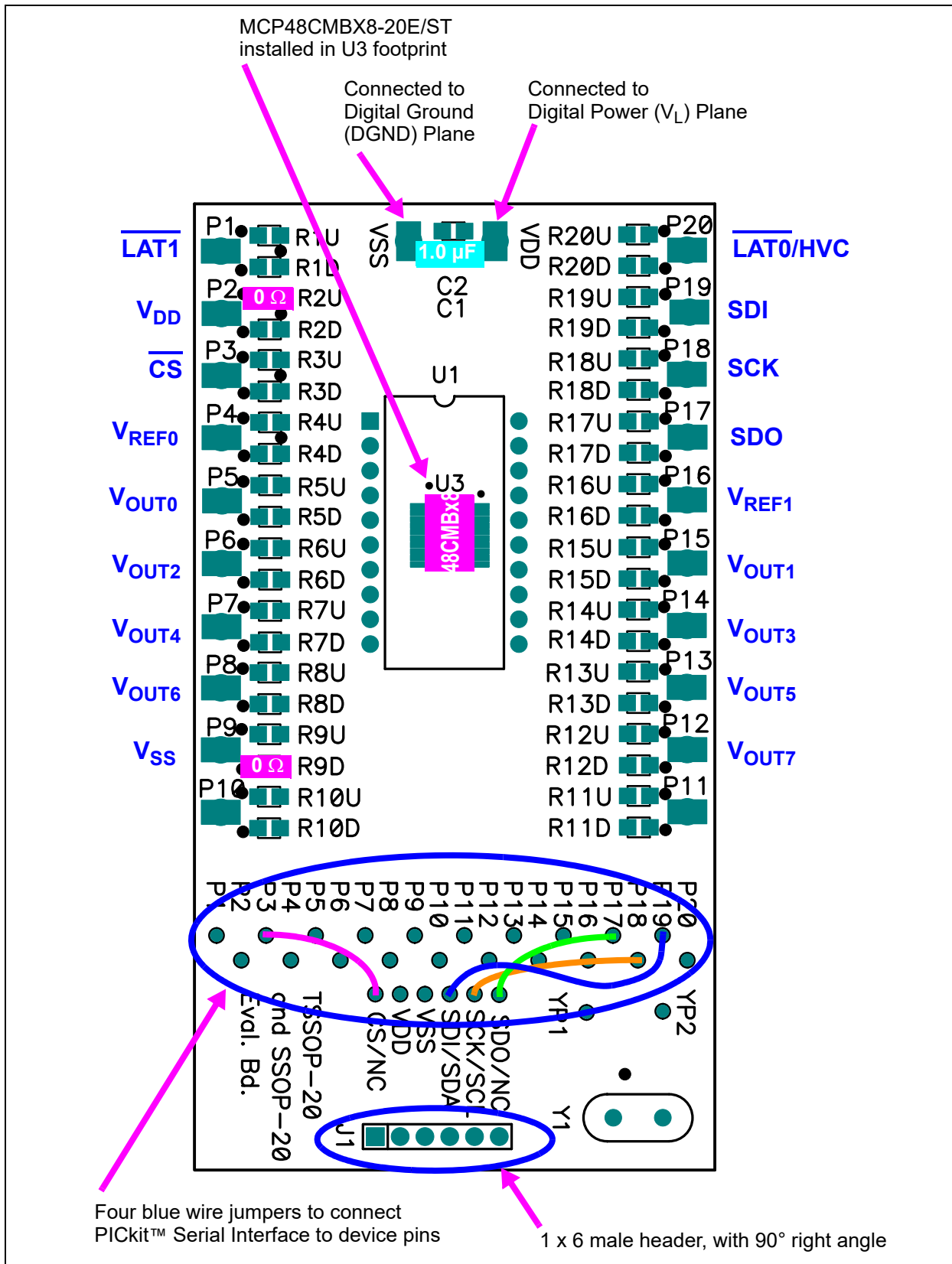
FIGURE 6-1: MCP48CXBX4/8 Evaluation Board Circuit Using TSSOP20EV.
