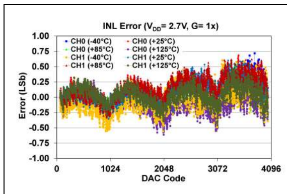
FIGURE 2-58: INL Error vs. DAC Code and Temperature (Dual-Channel - MCP48CXB22), V_{DD} = 2.7\text{V} , Gain = 1X.
