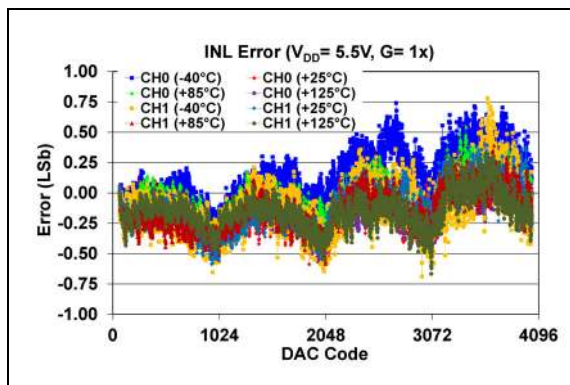
FIGURE 2-56: INL Error vs. DAC Code and Temperature (Dual-Channel - MCP48CXB22), V_{DD} = 5.5\text{V} , Gain = 1X.
