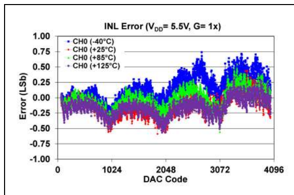
FIGURE 2-53: INL Error vs. DAC Code and Temperature (Single-Channel - MCP48CXB21), V_{DD} = 5.5\text{V} , Gain = 1X.
