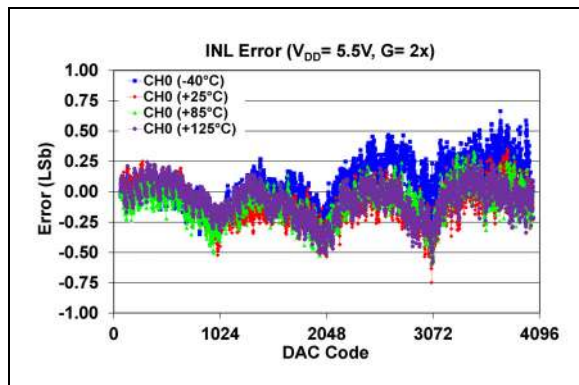
FIGURE 2-54: INL Error vs. DAC Code and Temperature (Single-Channel - MCP48CXB21), V_{DD} = 5.5\text{V} , Gain = 2X.
