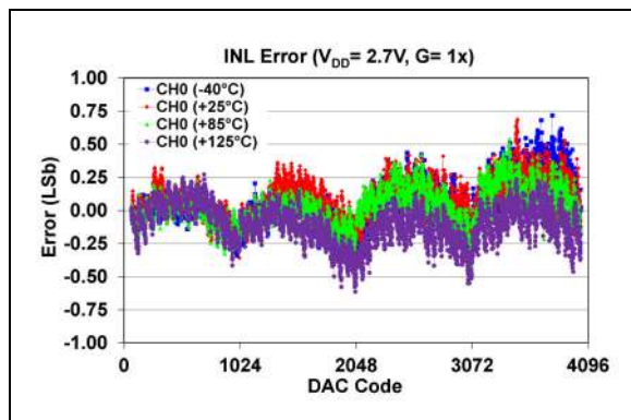
FIGURE 2-55: INL Error vs. DAC Code and Temperature (Single-Channel - MCP48CXB21), V_{DD} = 2.7\text{V} , Gain = 1X.
