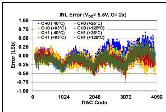
FIGURE 2-57: INL Error vs. DAC Code and Temperature (Dual-Channel - MCP48CXB22), V_{DD} = 5.5\text{V} , Gain = 2X.
