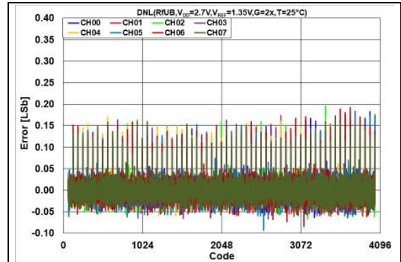
FIGURE 2-53: DNL Error vs. DAC Code and Temperature, V_{DD} = 2.7\text{V} , V_{REF} = 1.35\text{V} , T = +25^\circ\text{C} .
