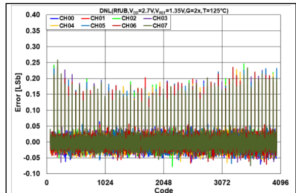
FIGURE 2-54: DNL Error vs. DAC Code and Temperature, V_{DD} = 2.7\text{V} , V_{REF} = 1.35\text{V} , T = +125^\circ\text{C} .
