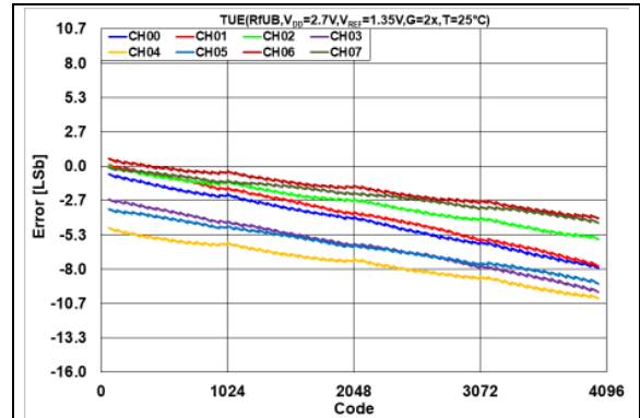
FIGURE 2-41: Total Unadjusted Error ( V_{OUT} ) vs. DAC Code and Temperature, V_{DD} = 2.7\text{V} , V_{REF} = 1.35\text{V} , T = +25^\circ\text{C} .
