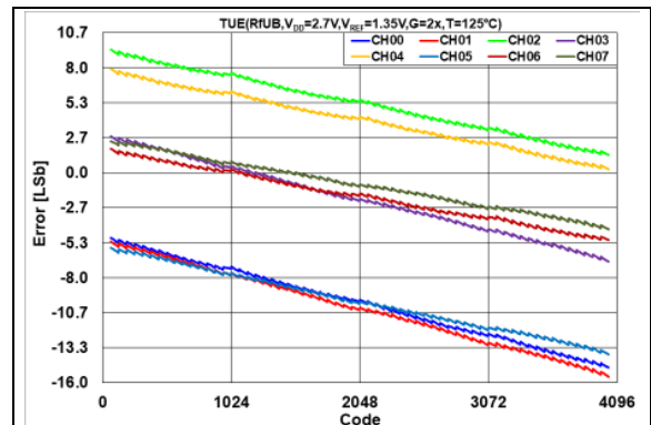
FIGURE 2-42: Total Unadjusted Error ( V_{OUT} ) vs. DAC Code and Temperature, V_{DD} = 2.7\text{V} , V_{REF} = 1.35\text{V} , T = +125^\circ\text{C} .
