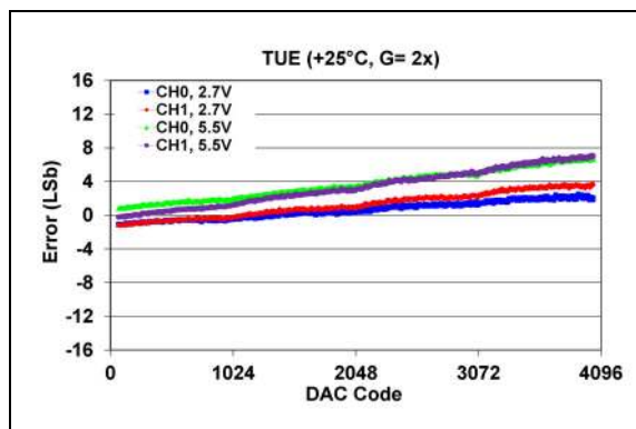
FIGURE 2-51: Total Unadjusted Error ( V_{OUT} ) vs. DAC Code, +25^\circ\text{C} , Gain = 2\text{X} .
