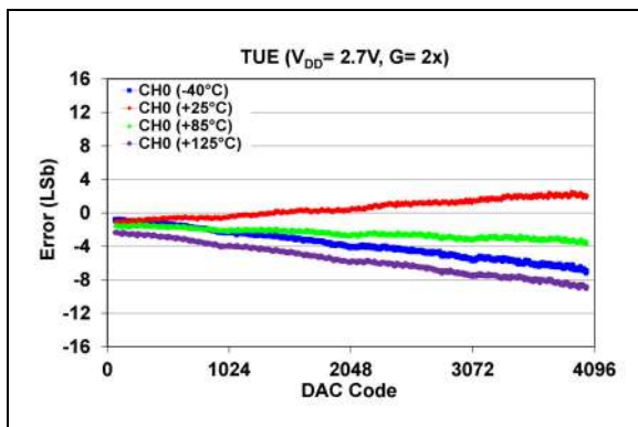
FIGURE 2-46: Total Unadjusted Error ( V_{OUT} ) vs. DAC Code and Temperature (Single-Channel - MCP48CXB21), V_{DD} = 2.7\text{V} , Gain = 2\text{X} .
