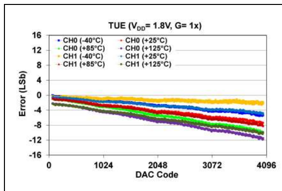
FIGURE 2-50: Total Unadjusted Error ( V_{OUT} ) vs. DAC Code and Temperature (Dual-Channel - MCP48CXB22), V_{DD} = 1.8\text{V} , Gain = 1\text{X} .
