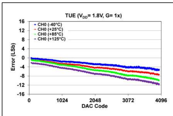
FIGURE 2-47: Total Unadjusted Error ( V_{OUT} ) vs. DAC Code and Temperature (Single-Channel - MCP48CXB21), V_{DD} = 1.8\text{V} , Gain = 1\text{X} .
