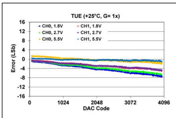
FIGURE 2-48: Total Unadjusted Error ( V_{OUT} ) vs. DAC Code, +25^\circ\text{C} , Gain = 1\text{X} .
