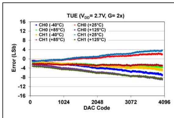
FIGURE 2-49: Total Unadjusted Error ( V_{OUT} ) vs. DAC Code and Temperature (Dual-Channel - MCP48CXB22), V_{DD} = 2.7\text{V} , Gain = 2\text{X} .
