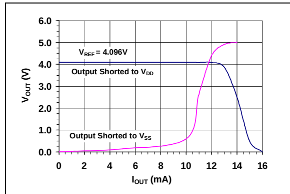
FIGURE 2-28: I_{OUT} vs. V_{OUT} . Gain = 2\times .
