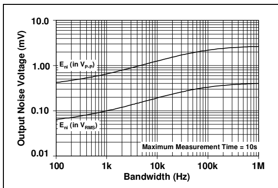
FIGURE 2-14: Output Noise Voltage ( V_{REF} Noise Voltage) vs. Bandwidth. Gain = 1\times .
