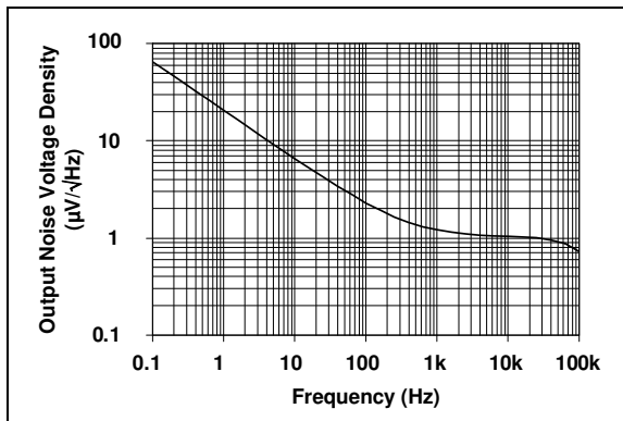
FIGURE 2-13: Output Noise Voltage Density ( V_{REF} Noise Density) vs. Frequency. Gain = 1\times .
