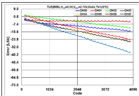
FIGURE 2-100: Total Unadjusted Error ( V_{OUT} ) vs. DAC Code, T = +125^\circ\text{C} , V_{DD} = 5.5\text{V} .
