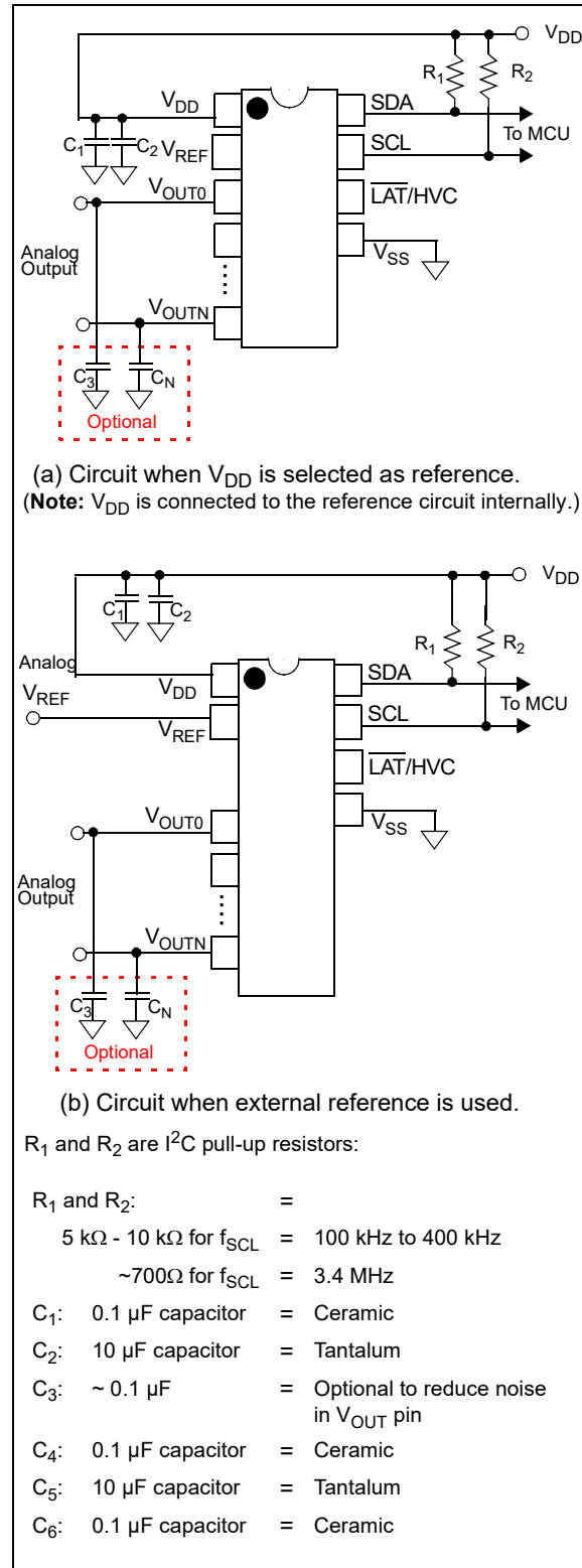
FIGURE 8-3: Circuit Example.
