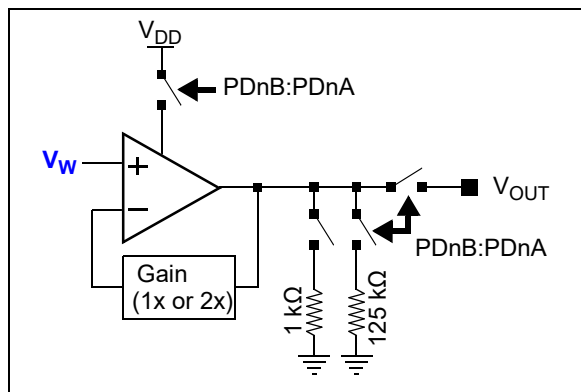
FIGURE 5-8: V_{OUT} Power-Down Block Diagram.
