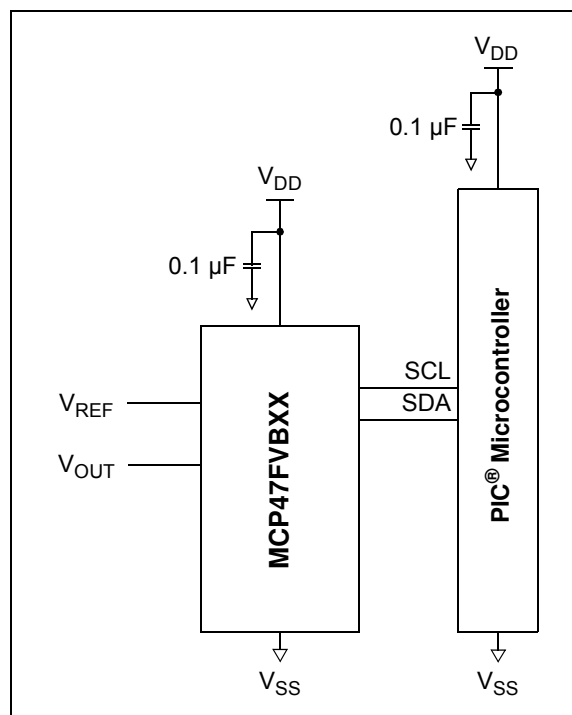
FIGURE 8-10: Typical Microcontroller Connections.
