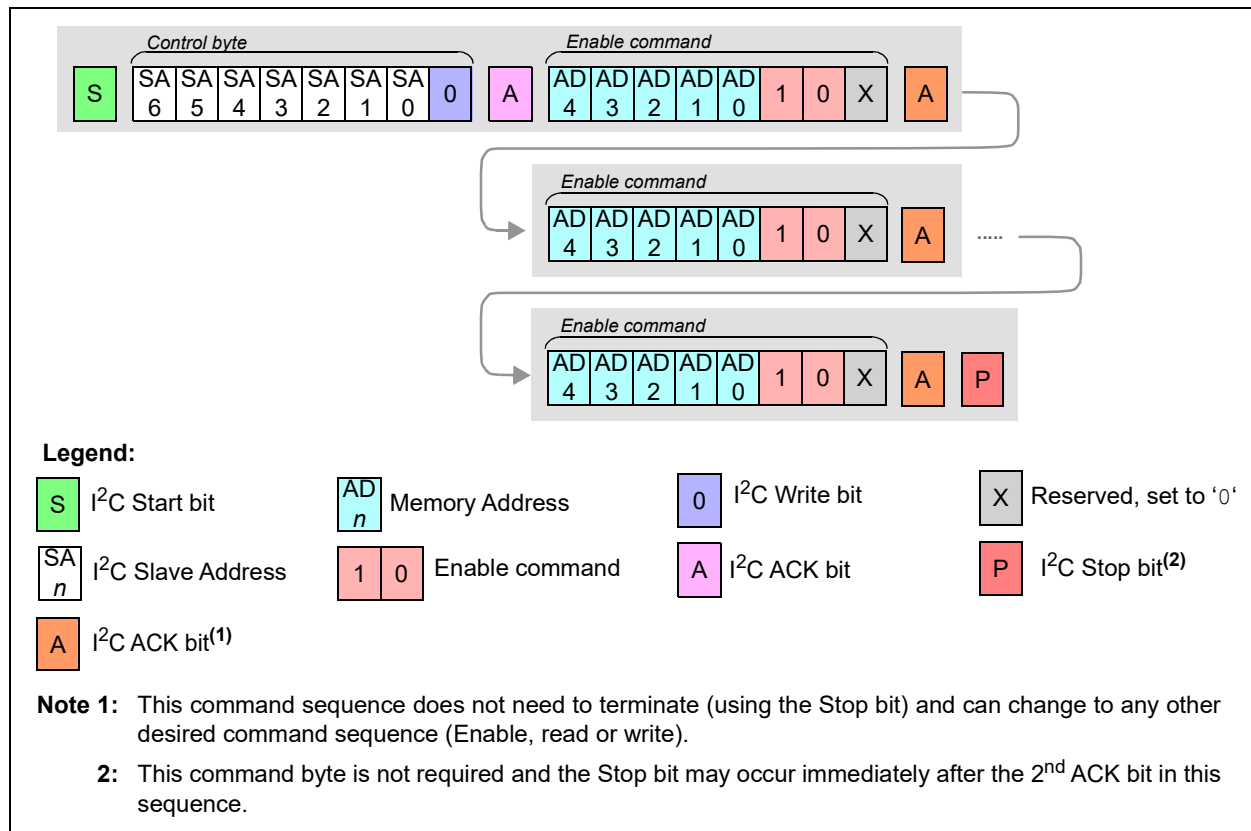
FIGURE 7-11: I²C Enable Command Sequence.
