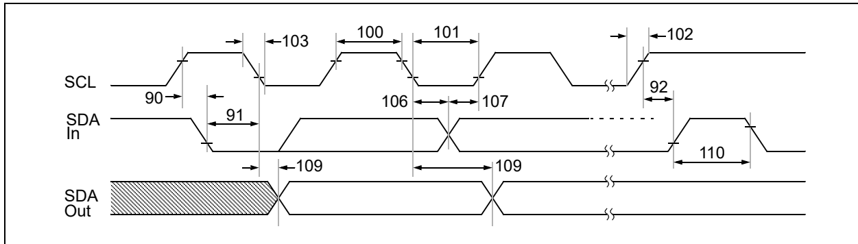
FIGURE 1-7: I 2 C Bus Timing Waveforms.
