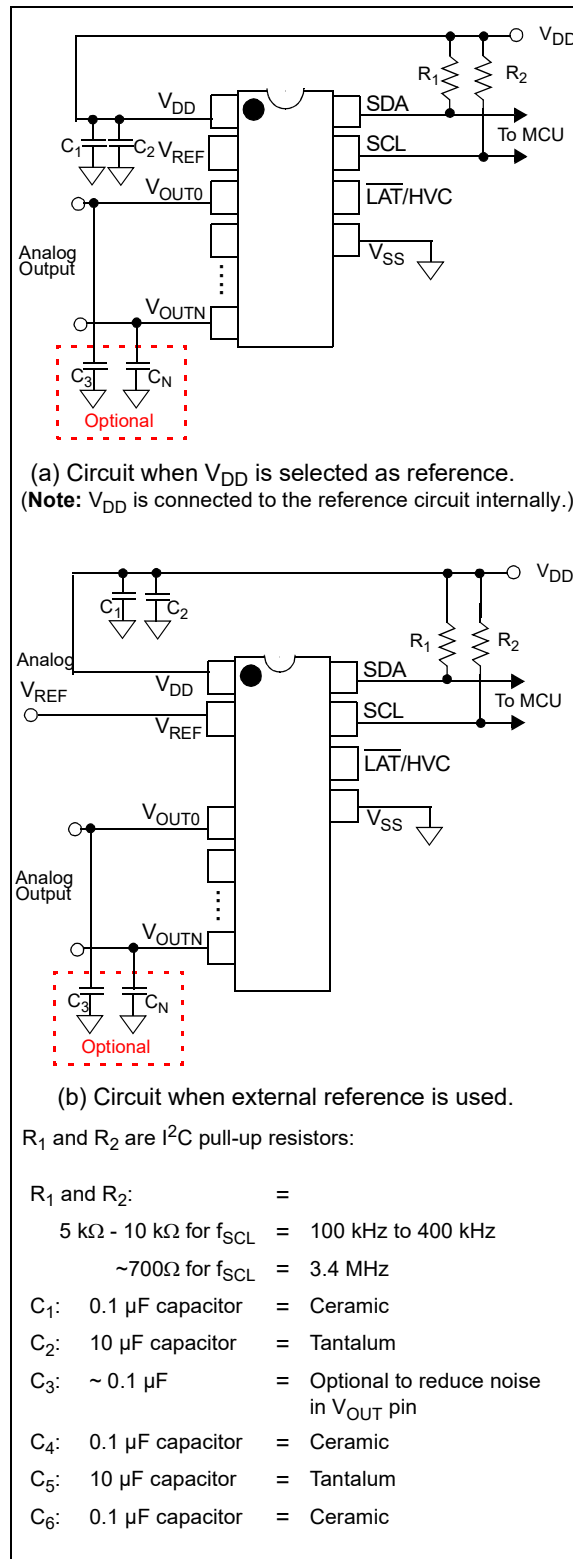
FIGURE 8-3: Circuit Example.
