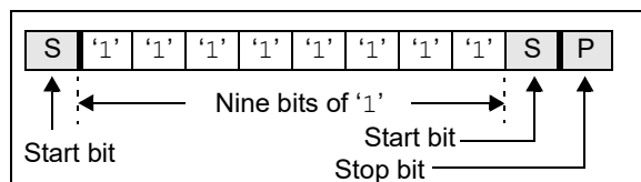
FIGURE 8-2: Software Reset Sequence Format.
