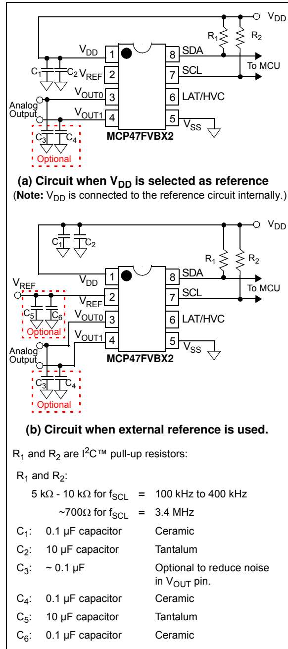
FIGURE 8-2: Example Circuit.
