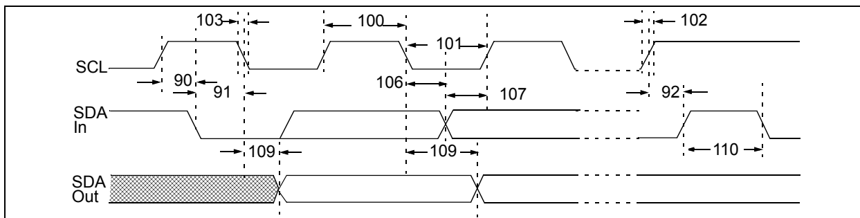
FIGURE 1-6: I²C™ Bus Timing Waveforms.
