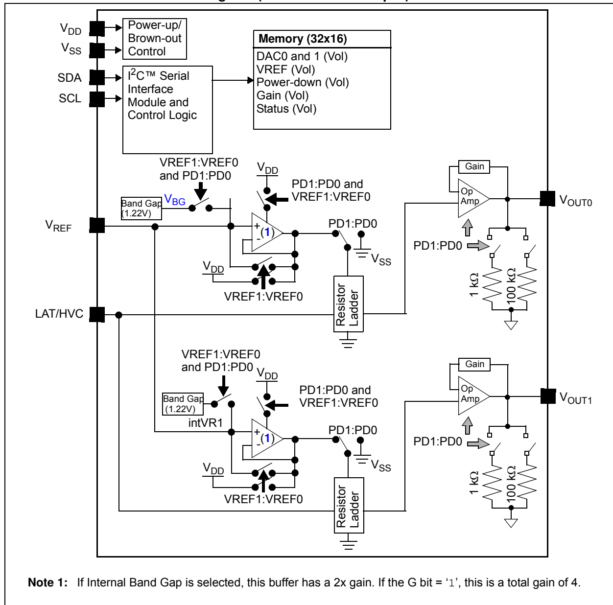
MCP47FVBX2 Device Block Diagram (Dual-Channel Output)
