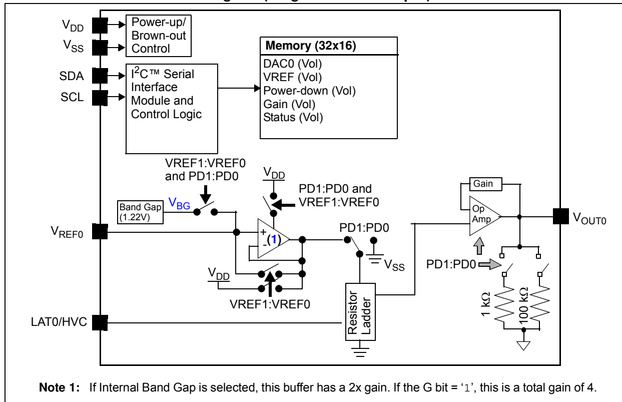
MCP47FVBX1 Device Block Diagram (Single-Channel Output)
