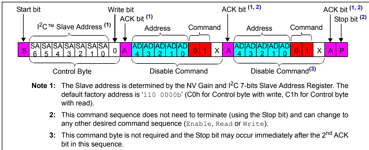
FIGURE 7-12: I²C Disable Command Sequence.
