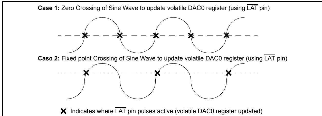
FIGURE 5-9: Example use of \overline{\text{LAT}} pin operation.
