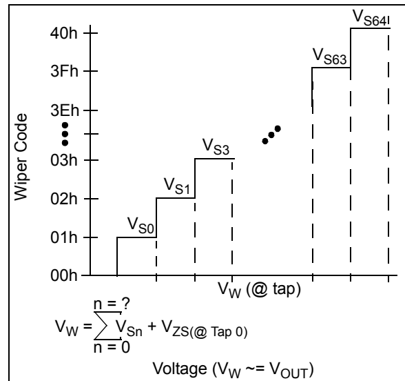
FIGURE C-1: V_W (V_{OUT}) .
