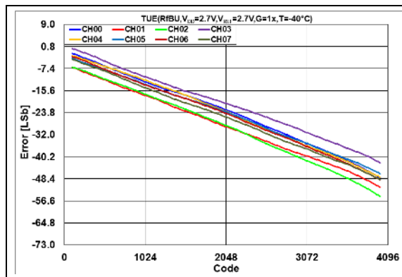
FIGURE 2-95: Total Unadjusted Error ( V_{OUT} ) vs. DAC Code, T = -40^\circ\text{C} , V_{DD} = 2.7\text{V} .
