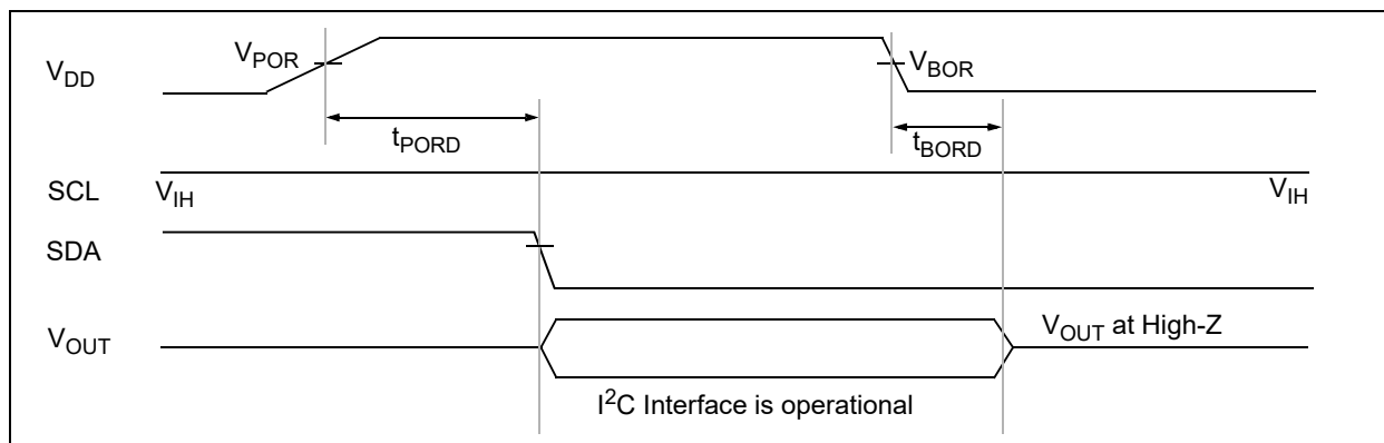
FIGURE 1-3: Power-on and Brown-out Reset Waveforms.
