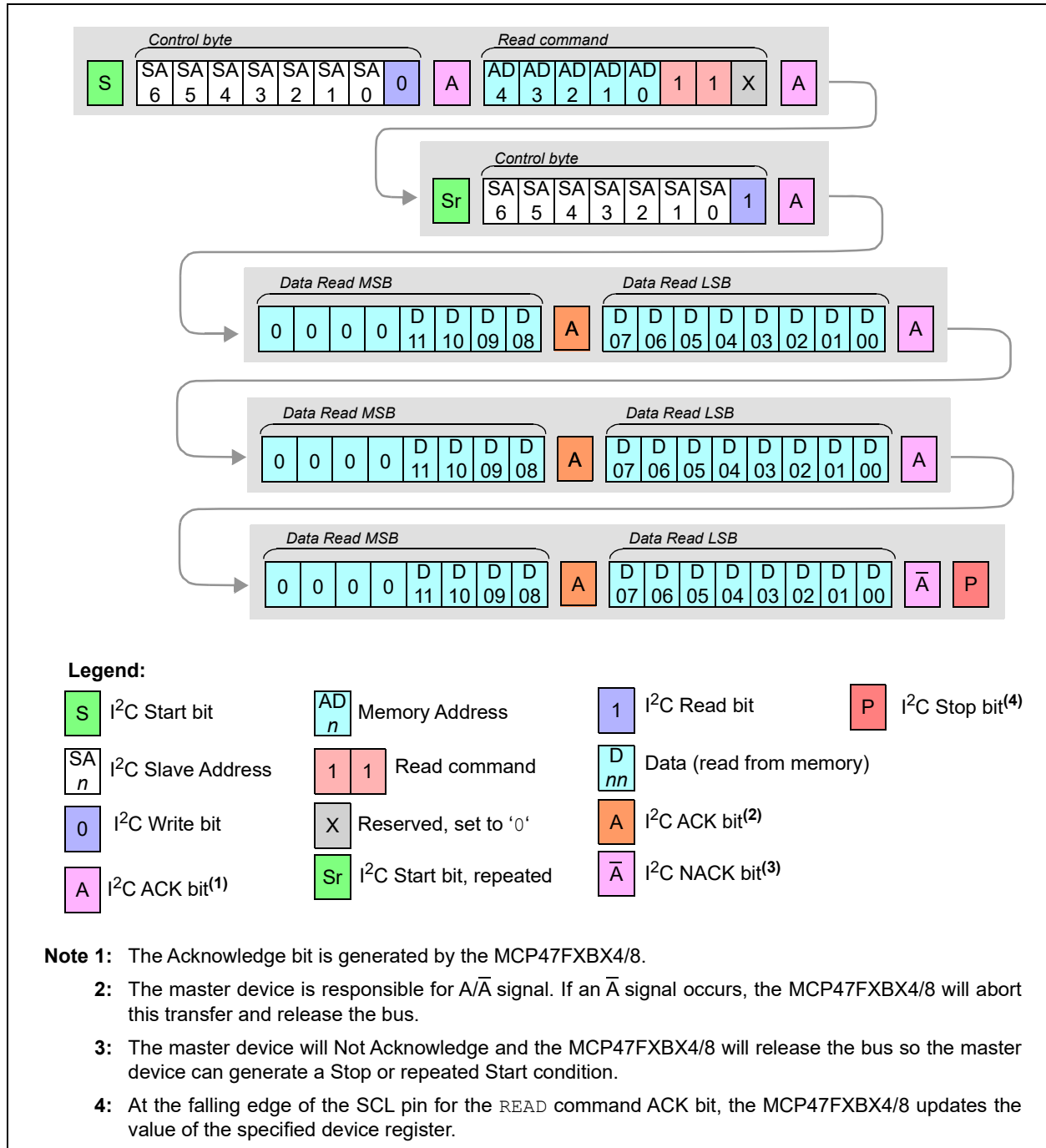
FIGURE 7-7: Continuous READ Command of Specified Address.
