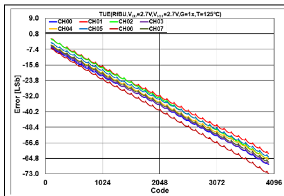
FIGURE 2-97: Total Unadjusted Error ( V_{OUT} ) vs. DAC Code, T = +125^\circ\text{C} , V_{DD} = 2.7\text{V} .
