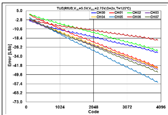
FIGURE 2-64: Total Unadjusted Error ( V_{OUT} ) vs. DAC Code, T = +125^\circ\text{C} , V_{DD} = 5.5\text{V} .
